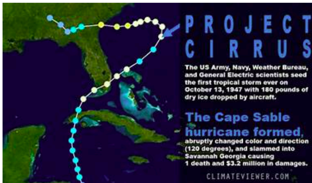
The modified path of a hurricane manipulated in Project Cirrus.
