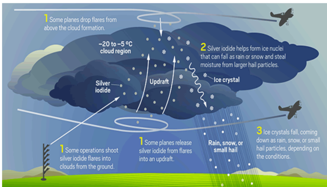
Explanation graphic detailing how cloud seeding works.
