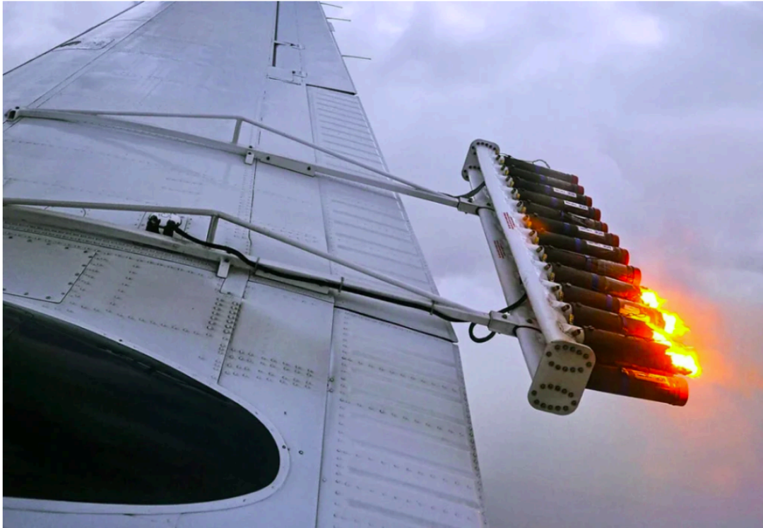
Cloud seeding with silver iodide.
